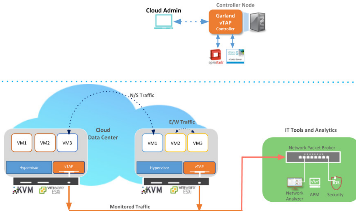
Figure 2. VMware/OpenStack Deployment
