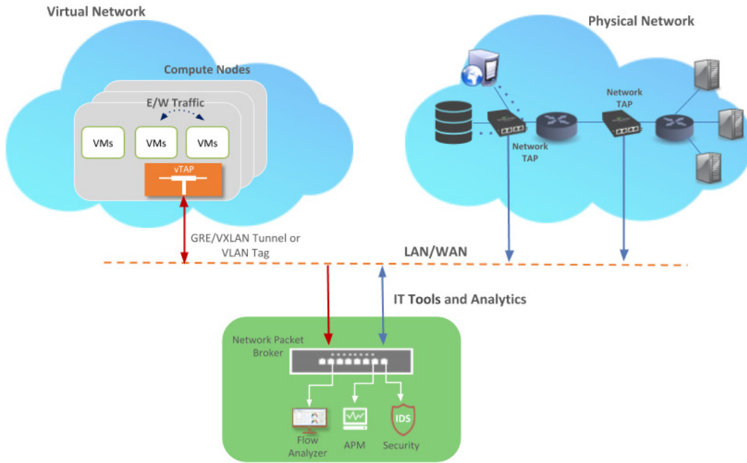
Figure 1. Hybrid Deployment
